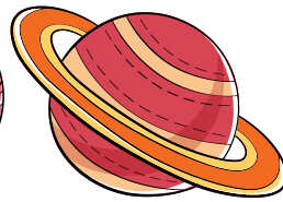
SATURN
