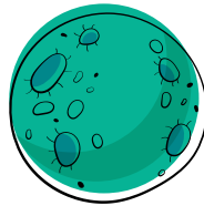
MERCURY
