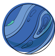
NEPTUNE
